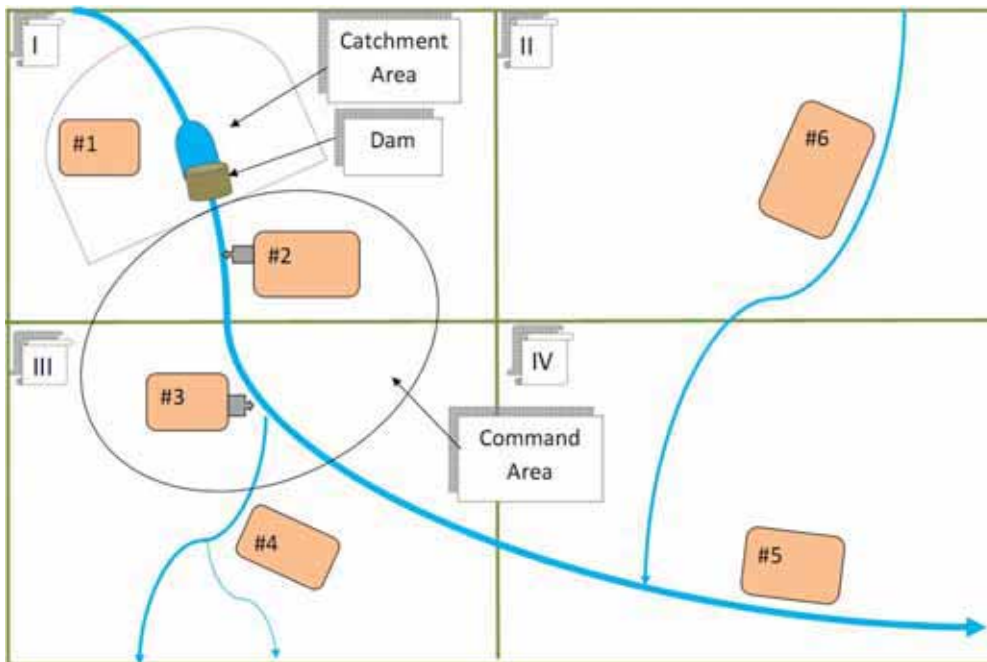
Figure 2: Large Dams
